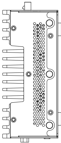
Right View
