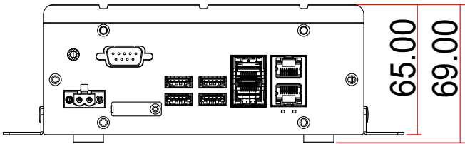
Front View
