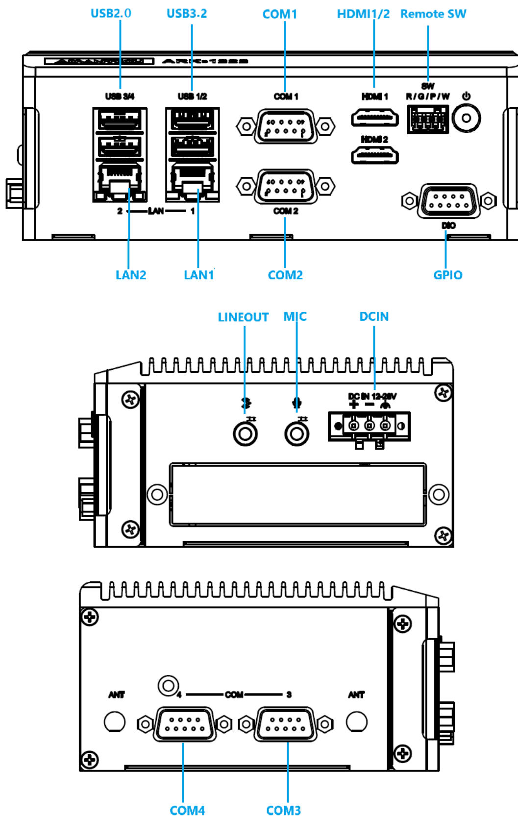
Figure 2.1 ARK-1222 Front and Side I/O Connector Diagram
