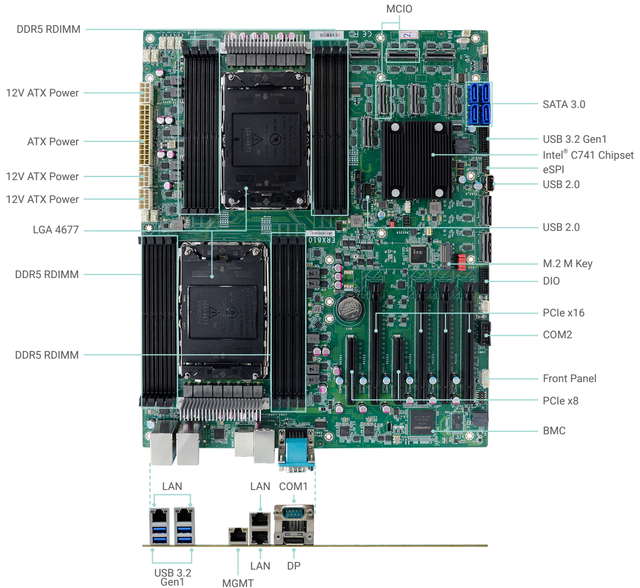
Top View
