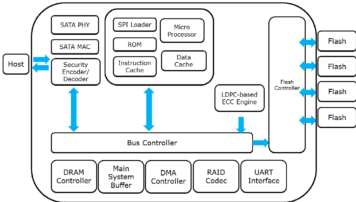
Figure 3: Innodisk M.2 (S80) 3MG5-P Block Diagram
