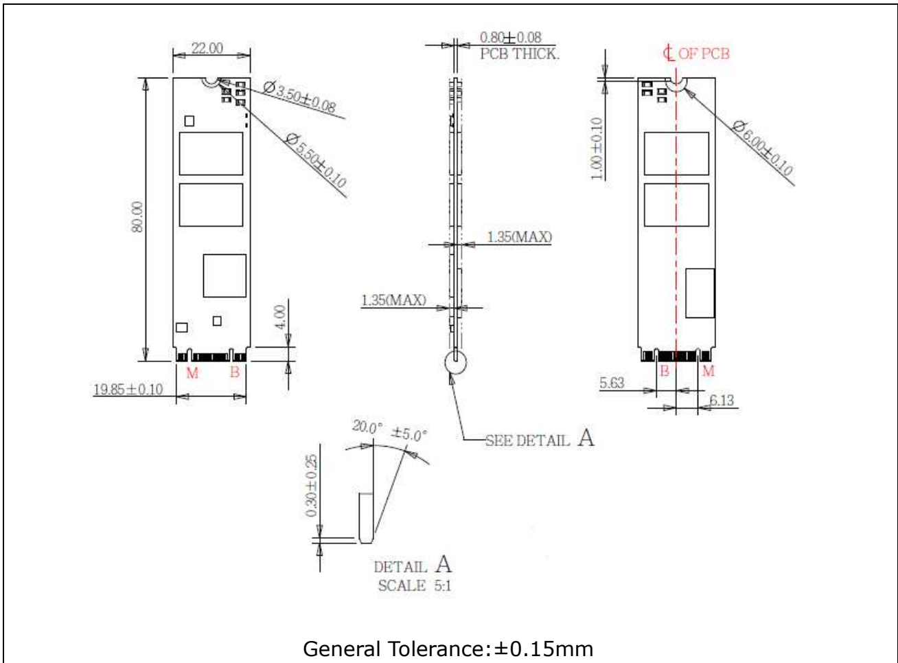
Figure 2: M.2 (S80) 3MG5-P mechanical diagram
