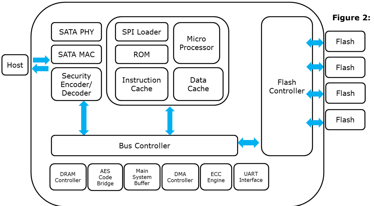
Innodisk 1.8" SATA SSD 3SE2-P with AES Block Diagram
