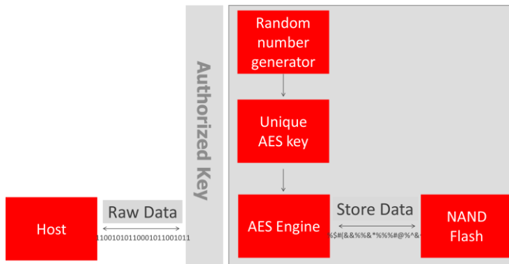
Figure 3: Innodisk 1.8" SATA SSD 3SE2-P AES flow chart
