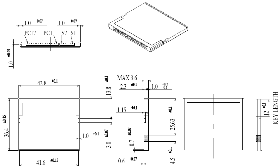
Figure 4: CFast D150Q mechanical dimensions
