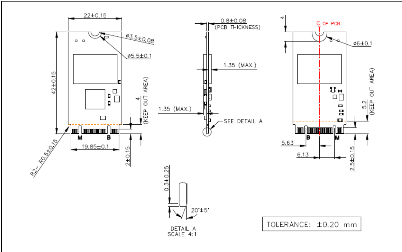
Figure 2: Innodisk M.2 (S42) 3SE4 diagram
