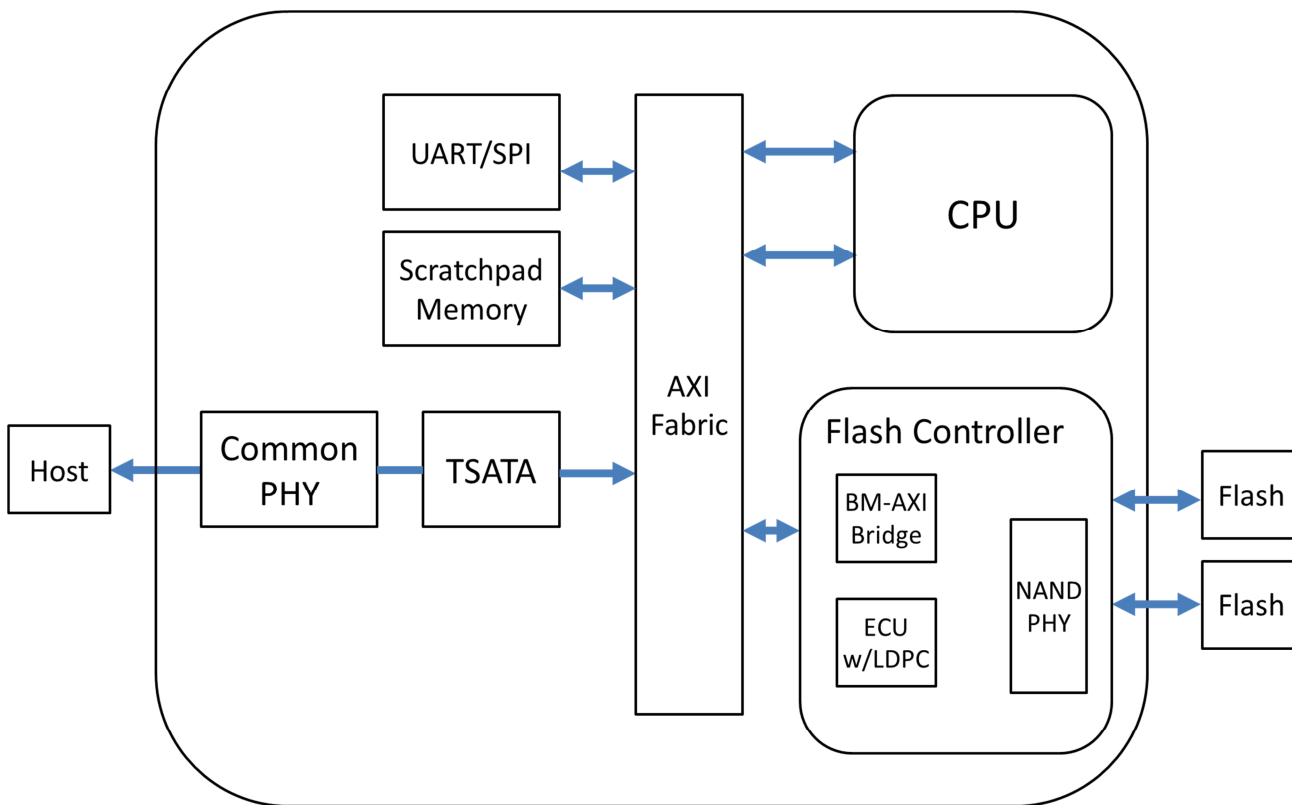
Figure 3: Innodisk M.2 (S80) 3SE4 Block Diagram
