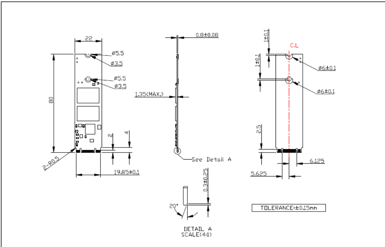
Figure 2: Innodisk M.2 (S80) 3SE4 diagram
